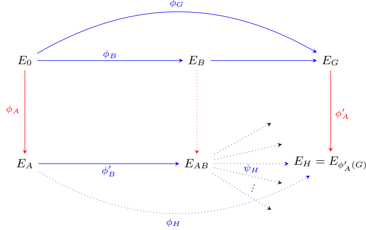
Fig. 3: Computing the action of \phi_A on G .
